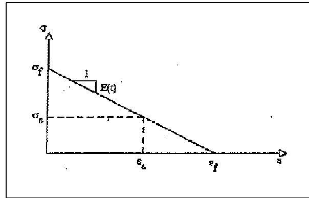
Figure A2-1. Cracking failure surface and \epsilon_f generation from the slow load fracture data
