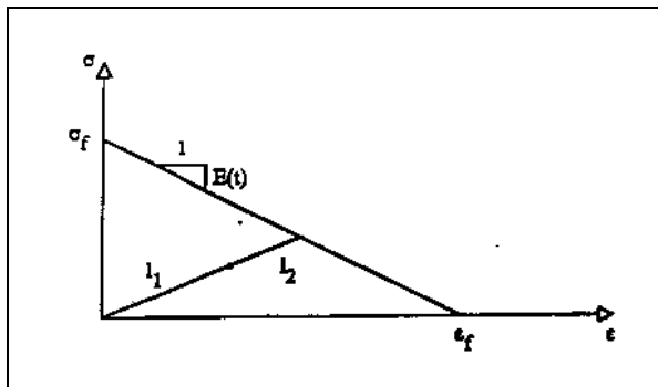
Figure A2-3. Cracking potential generation for a specific cracking failure surface
