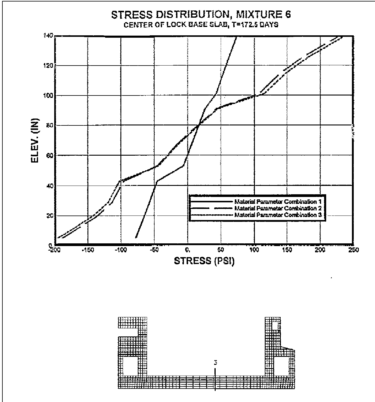
Figure A-7. Section plot example
