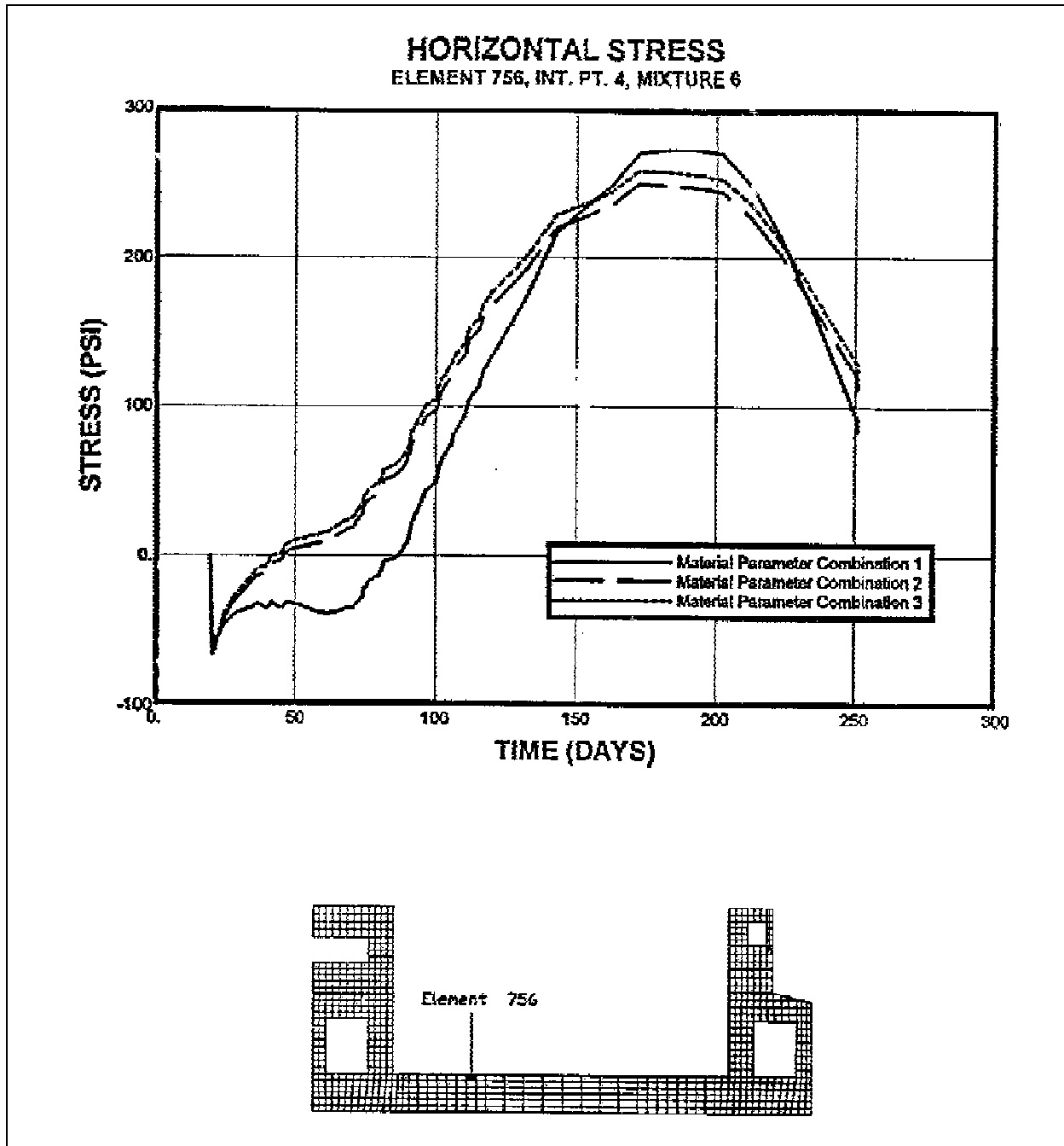
Figure A-6. Stress time-history plot example
