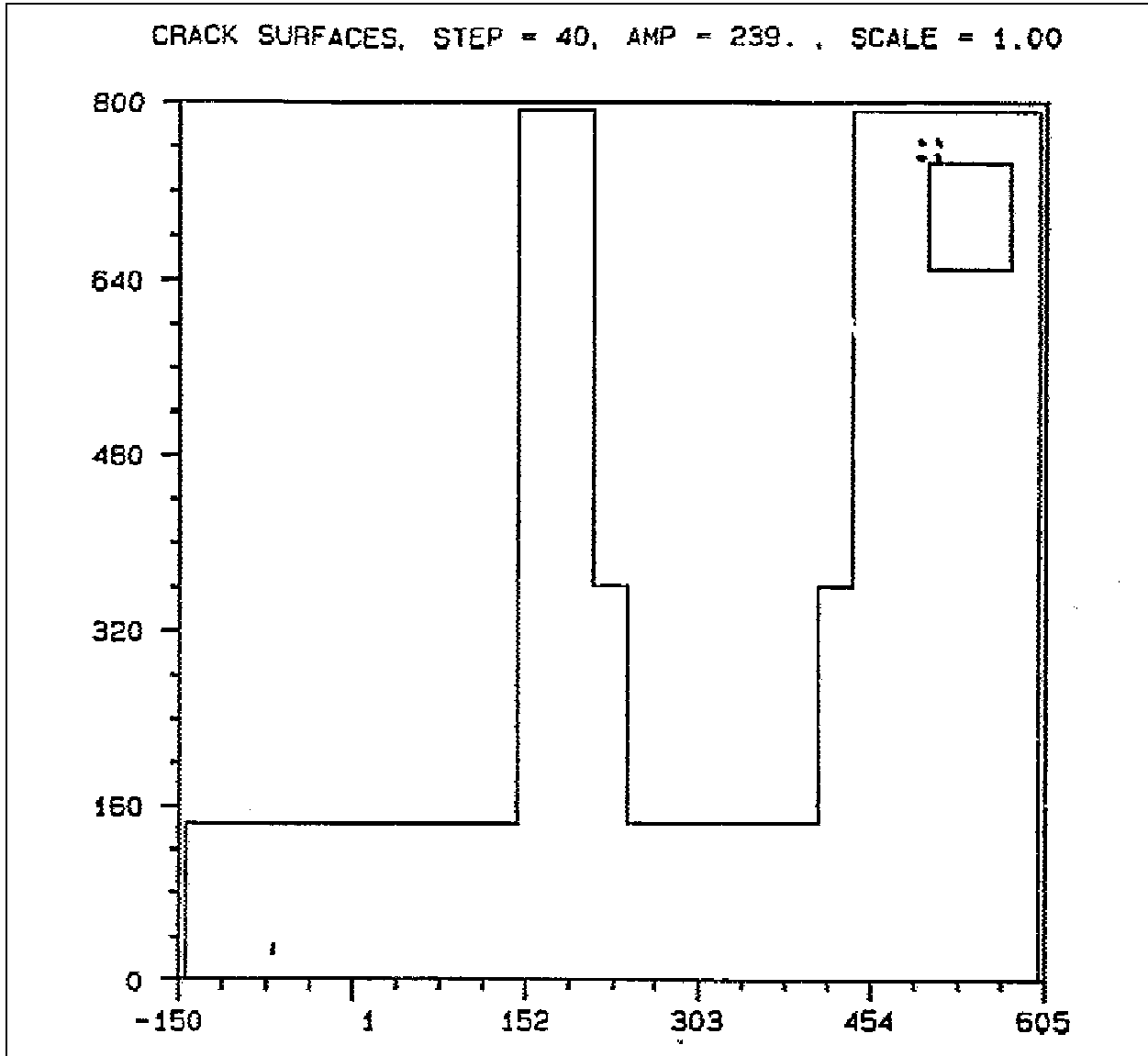
Figure A-9. Cracked location plot example
