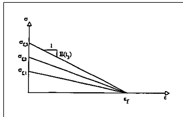
Figure A2-2. Computer generated, time-dependent (aging modulus) cracking failure surfaces
