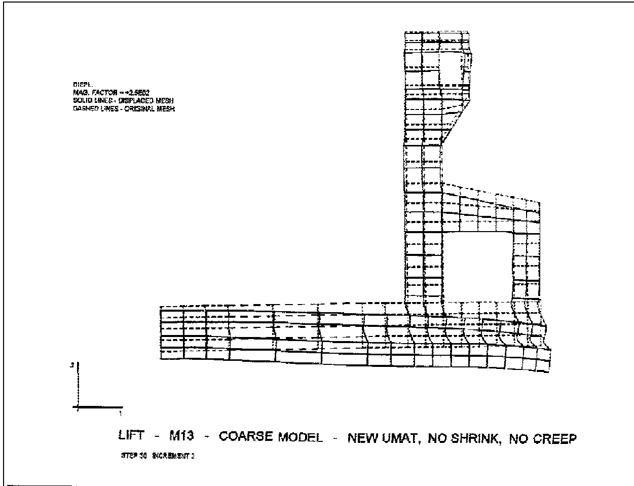
Figure A-8. Displaced shape plot example
