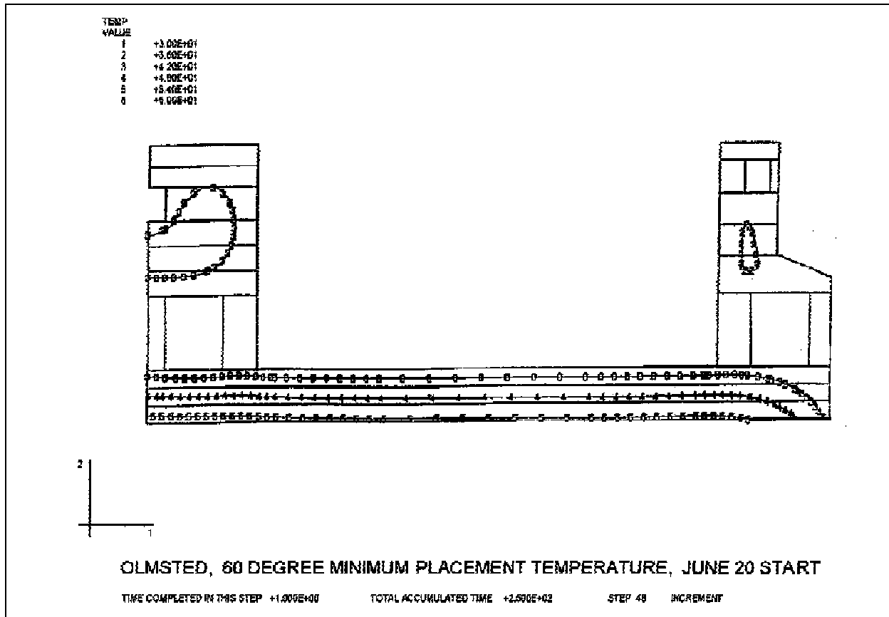
Figure A-4. Temperature contour plot example
