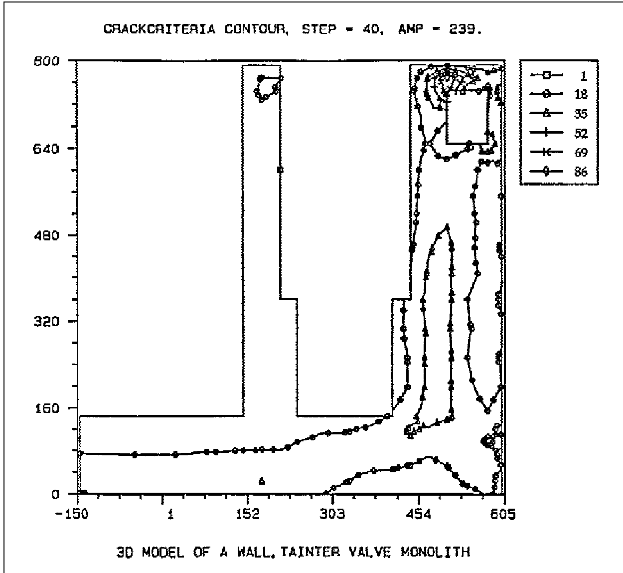
Figure A-5. Crack potential contour plot example
